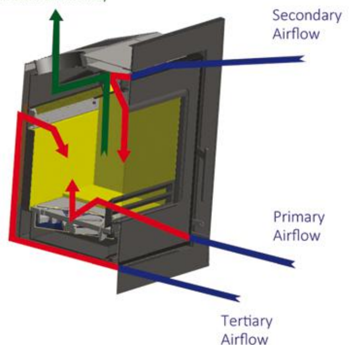
Double Baffle Efficiency
